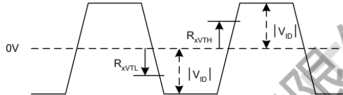
Differential signals
