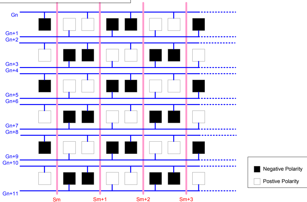
2-dot Inversion, INVSEL="L" & GOSEQ="L"
