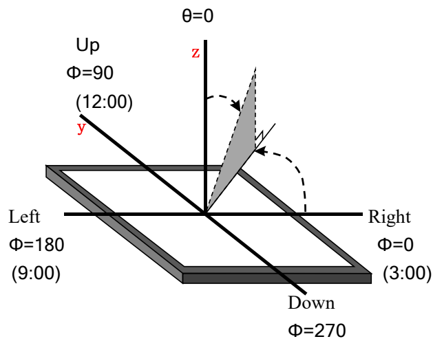
FIG.3.The definition of viewing angle
