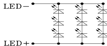
LED CIRCUIT DIAGRAM
