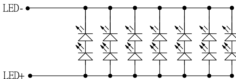
Figure: LED connection of backlight(Constant Current)
