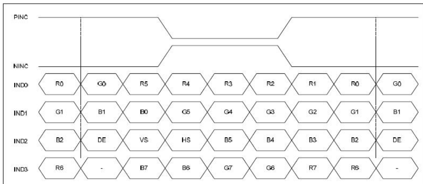
Figure 5.2.3: 8-bit LVDS input
