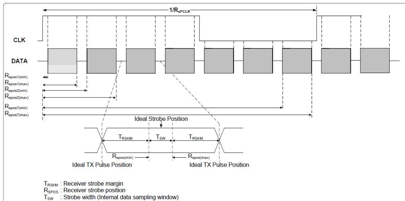
Figure 5.2.2: LVDS figure
