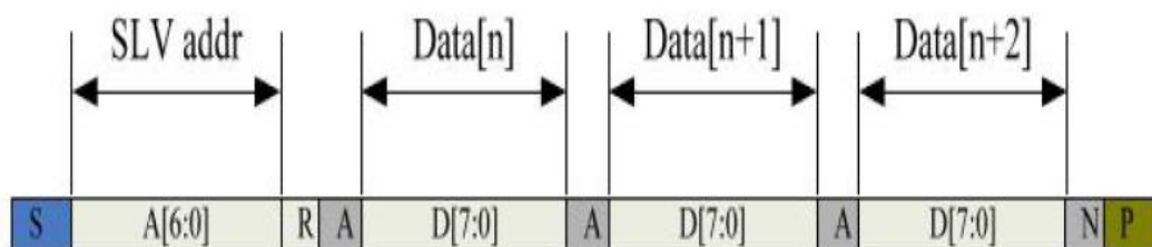
Figure 2-6 I2C master read, slave write
