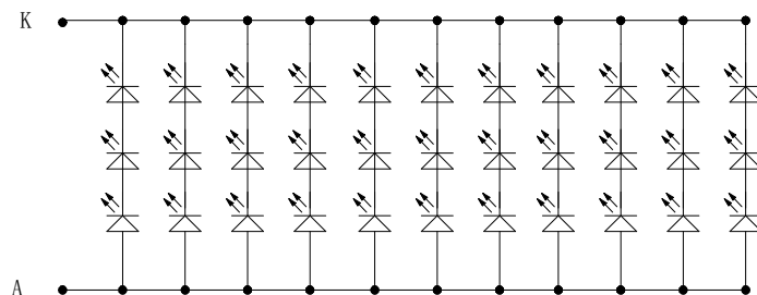
Figure: LED connection of backlight (Constant Current)
