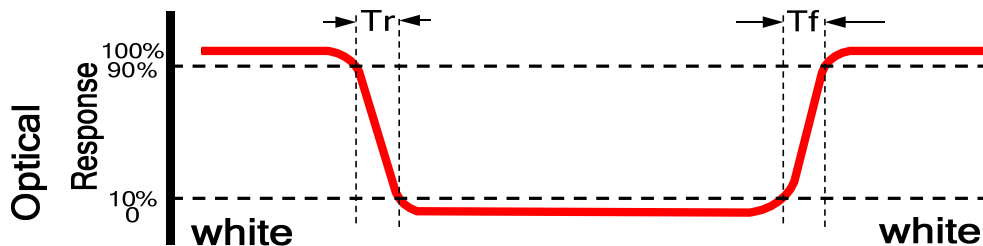
FIG.1. The definition of response Time
