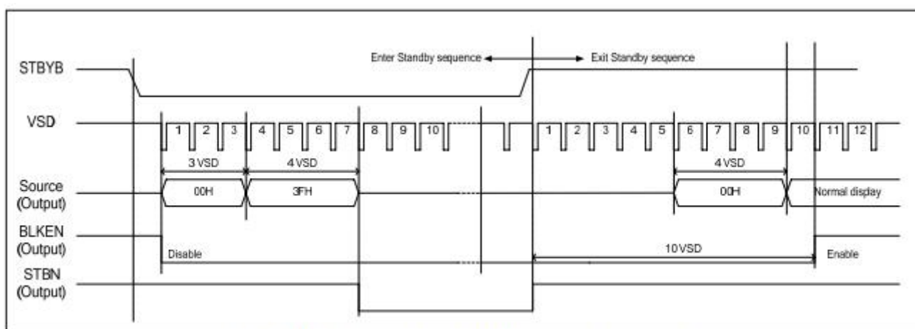
Figure 9.2: Enter and exit standby mode sequence
