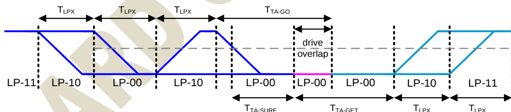
Figure 7.38: Turnaround Procedure
