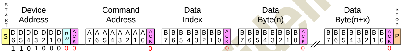
Figure 7.4: I2C Write Command + Data transmitter
