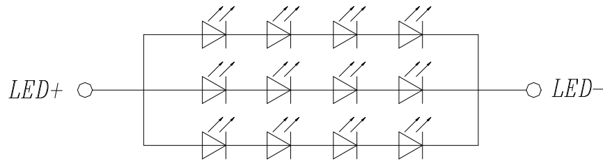
Figure: LED connection of backlight(Constant Current)
