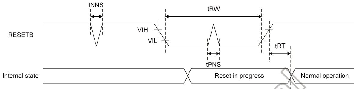
Figure 9.8: Reset timing
