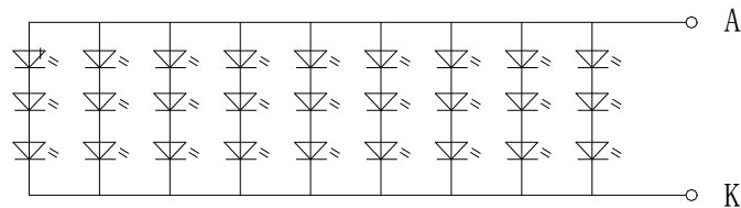
Figure: LED connection of backlight(Constant Current)
