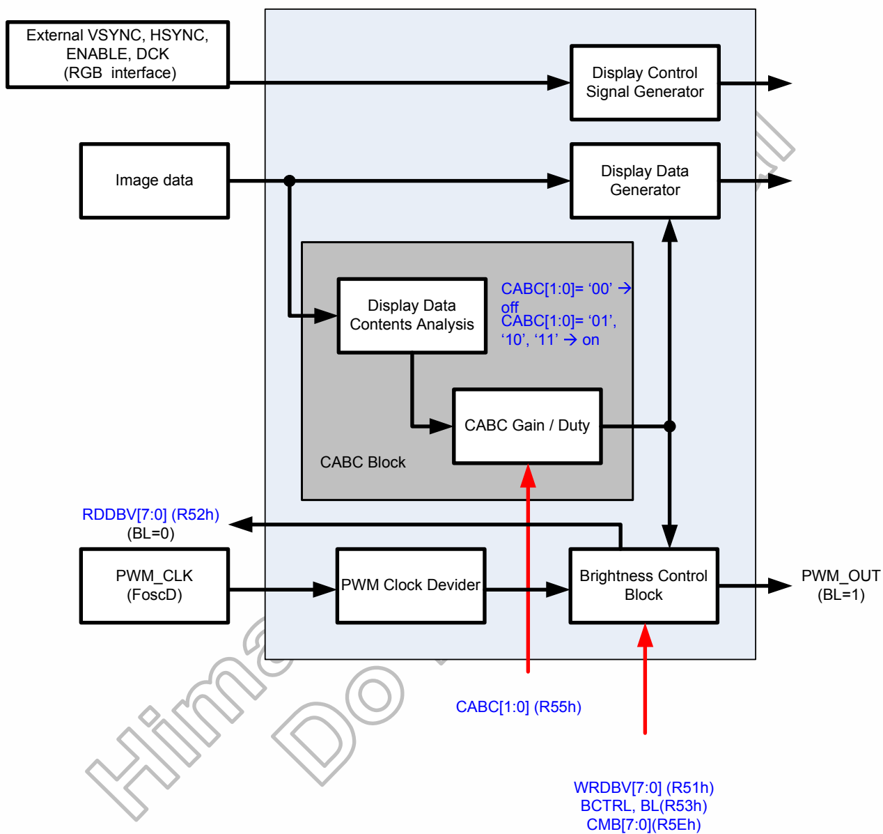
Figure 5.14: CABC Block Diagram
