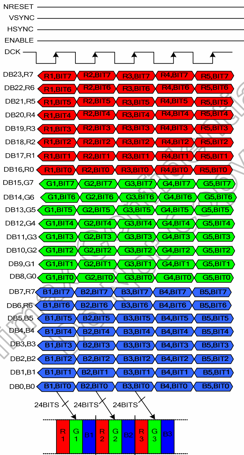
Figure 4.9: 24bit/pixel Color Order on the RGB I/F
