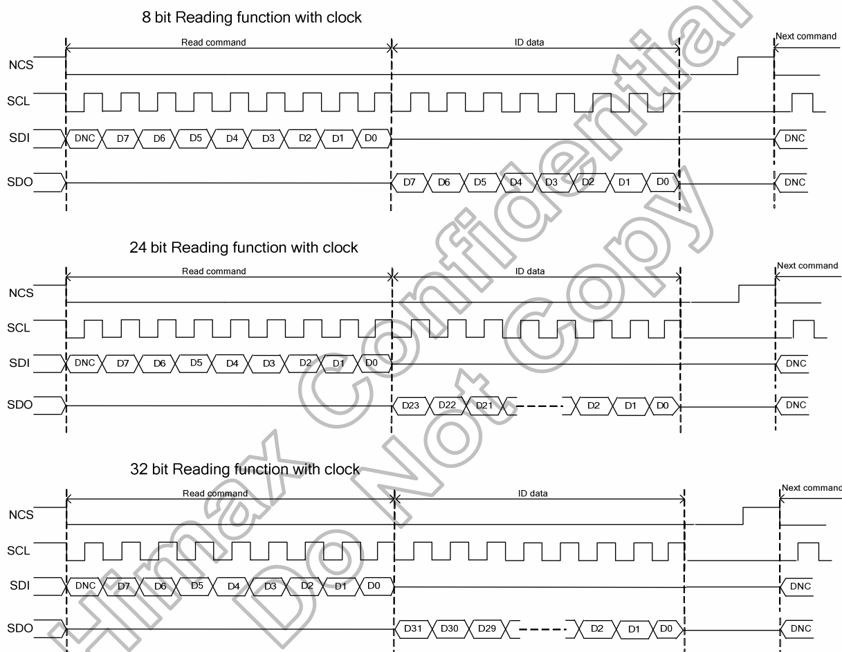
Figure 4.3 : 3 wire Serial Interface protocol, read mode
