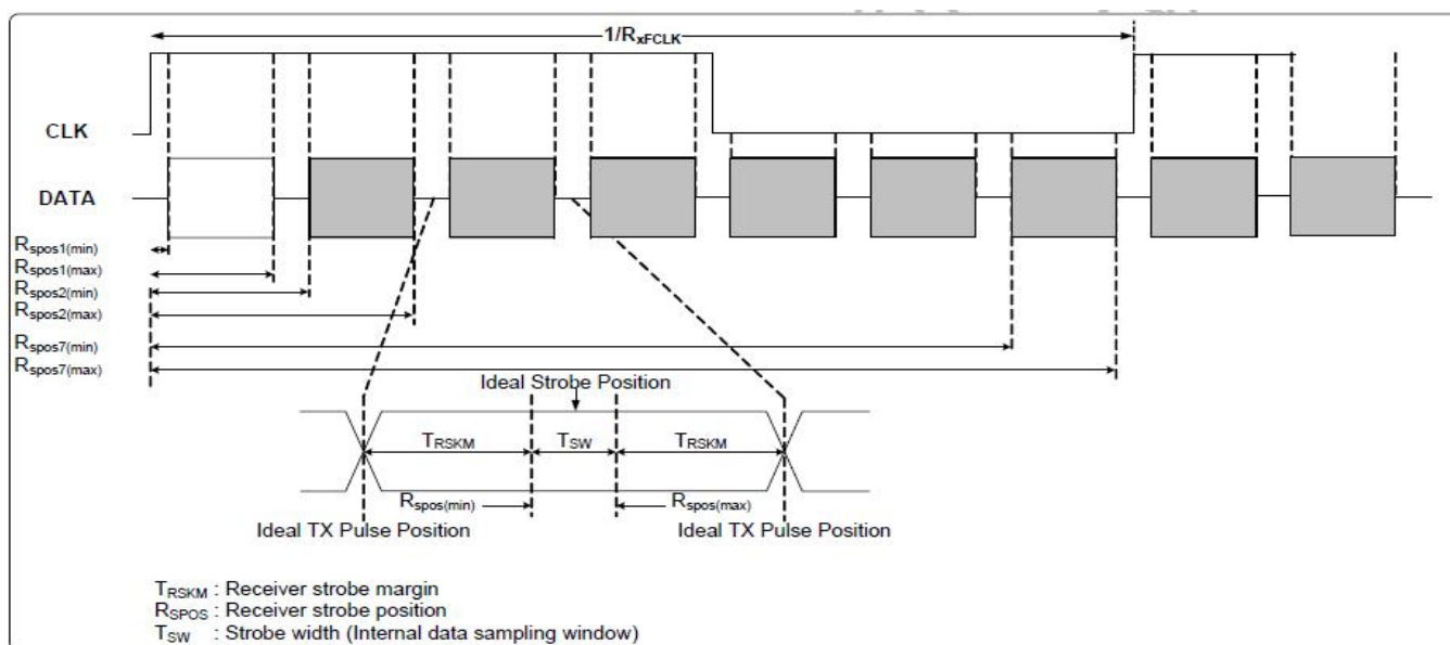
LVDS FIGURE
