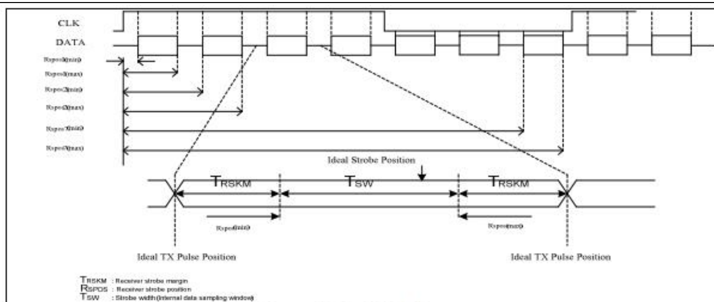
Figure 13.3: LVDS figure
