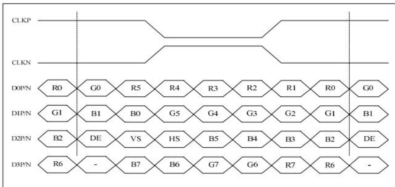
8-bit LVDS input(LVBIT=H, LVFMT=H)
