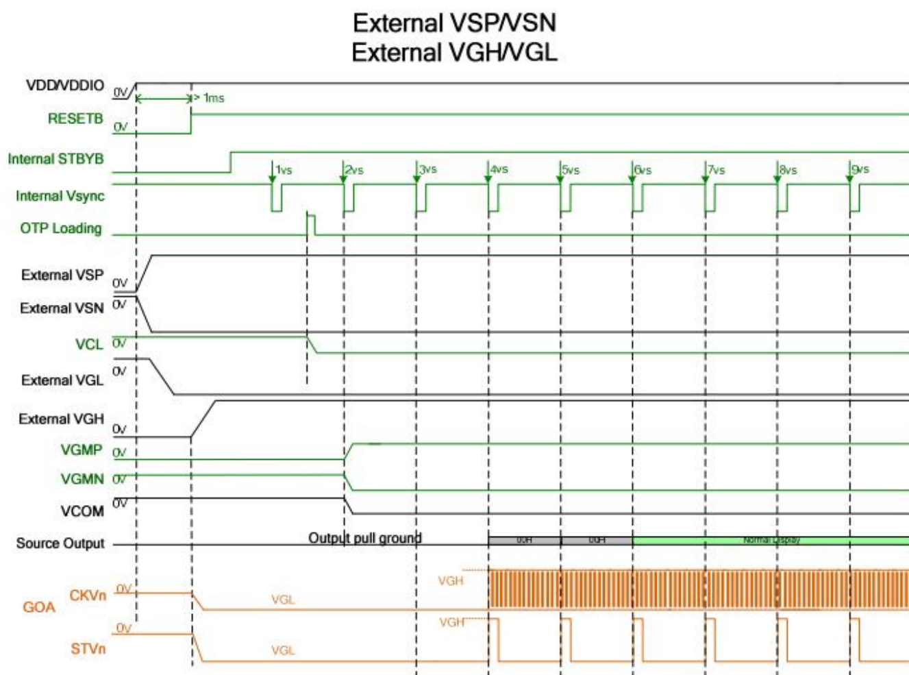
Power on sequence with PMODE=H
