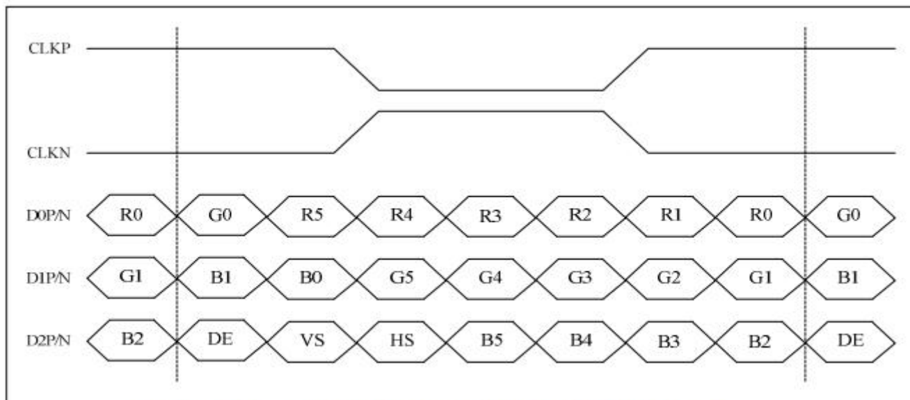
6-bit LVDS input (LVBIT=L, LVFMT=Don't care)
