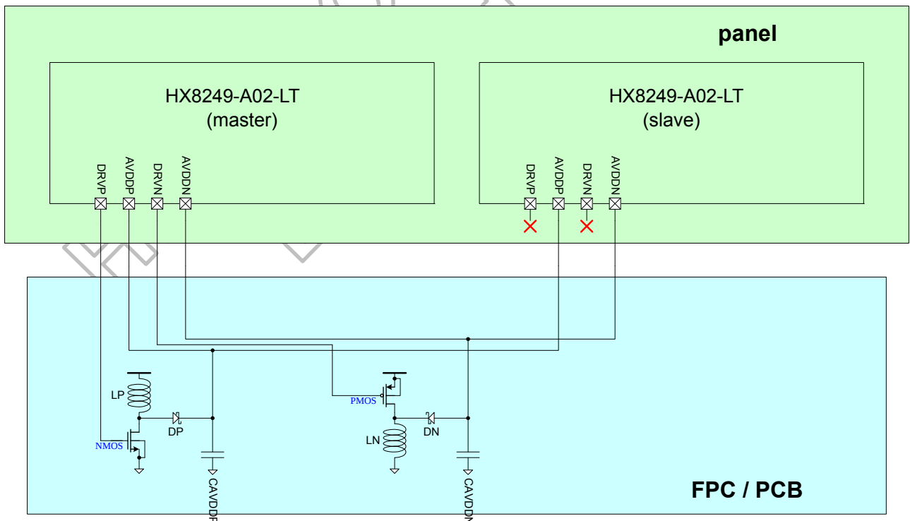
Figure 5.11: Cascade design for PFM
