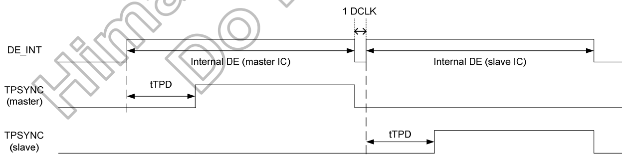
Figure 9.3: TPSYNC timing adjustment
