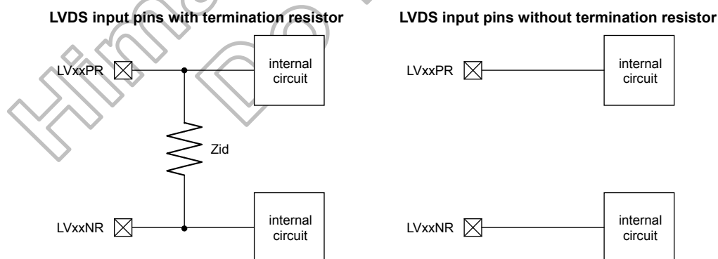
Figure 4.4: LVDS termination resistor selection
