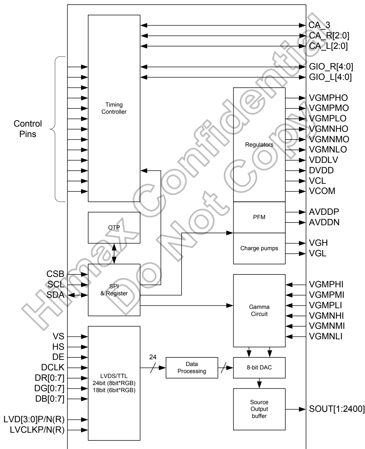
Figure 3.1: Block diagram
