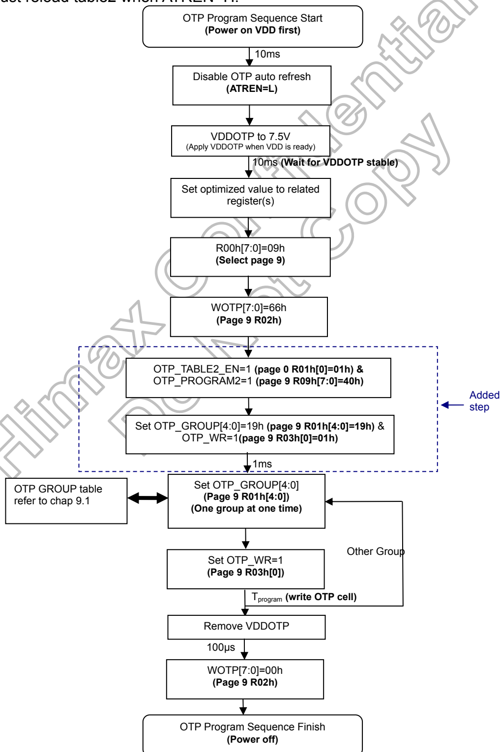
Figure 6.19: OTP 2nd program sequence (OTP table2)
