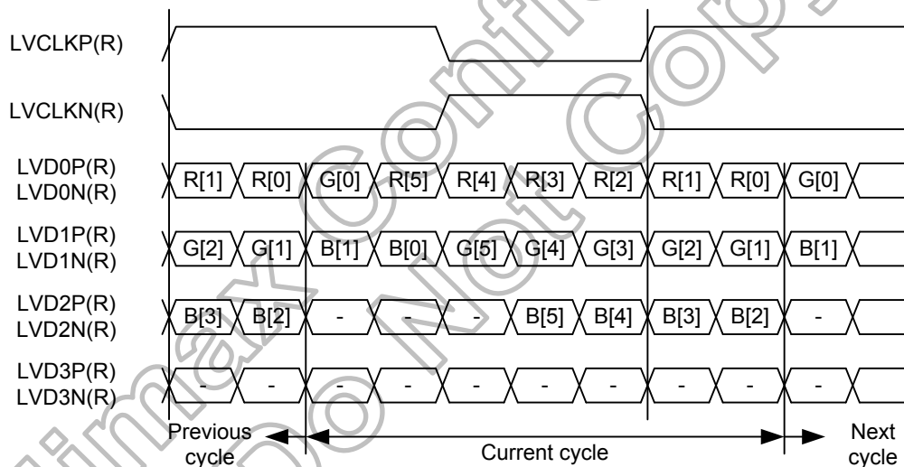
Figure 4.1: LVDS 6-bit
