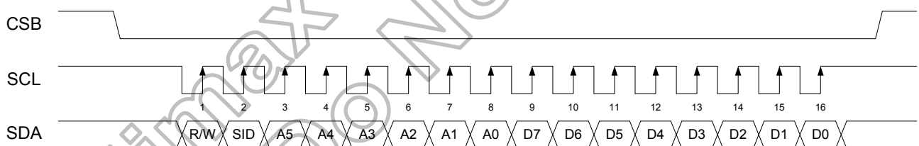
Figure 6.14: SPI format
