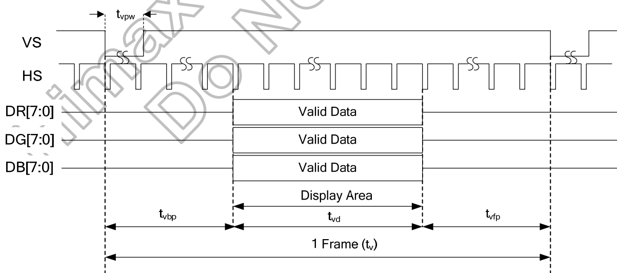
Figure 7.8: Vertical input timing at Sync mode
