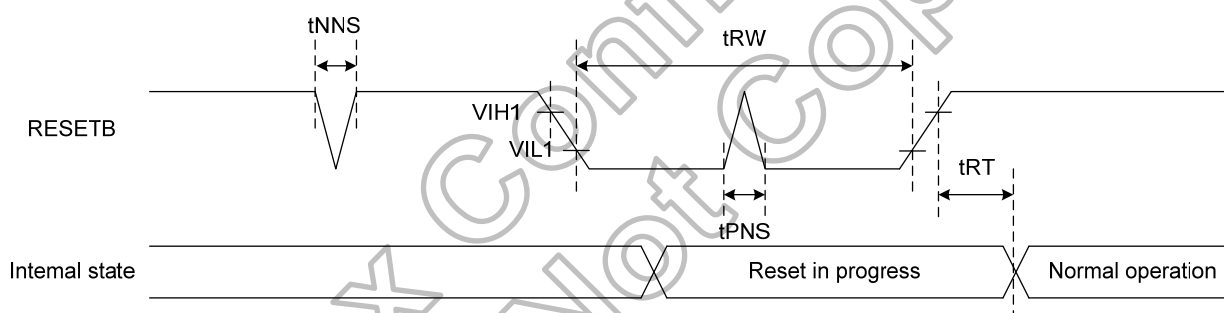
Figure 7.5: Reset timing
