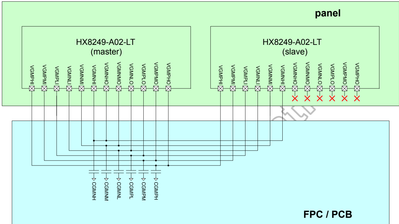
Figure 5.10: Cascade design for gamma reference voltages
