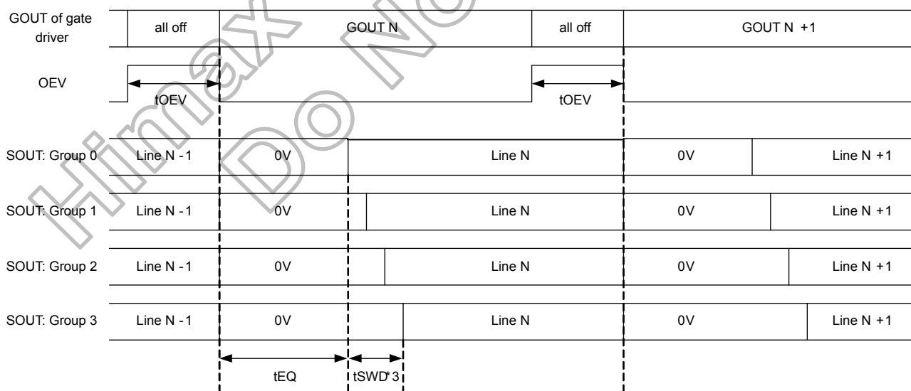
Figure 9.2: Source output timing
