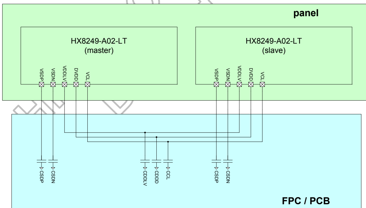
Figure 5.9: Cascade design for regulator outputs
