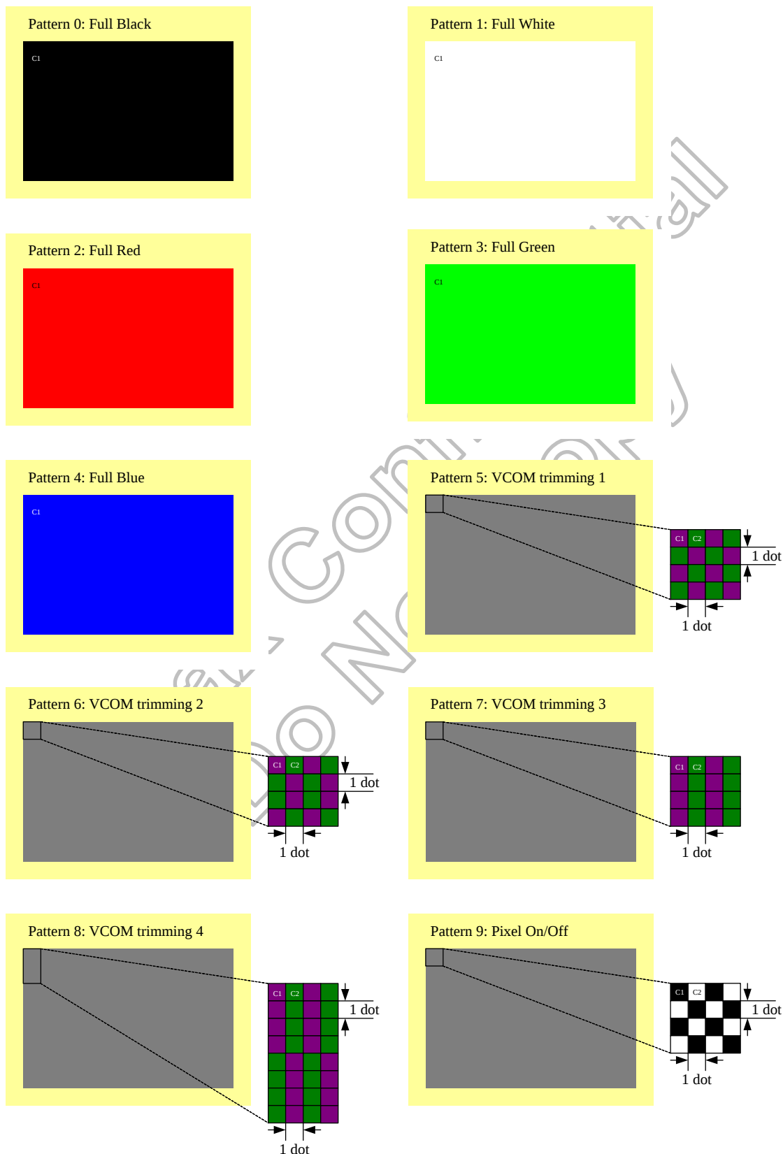
Figure 6.5: BIST patterns
