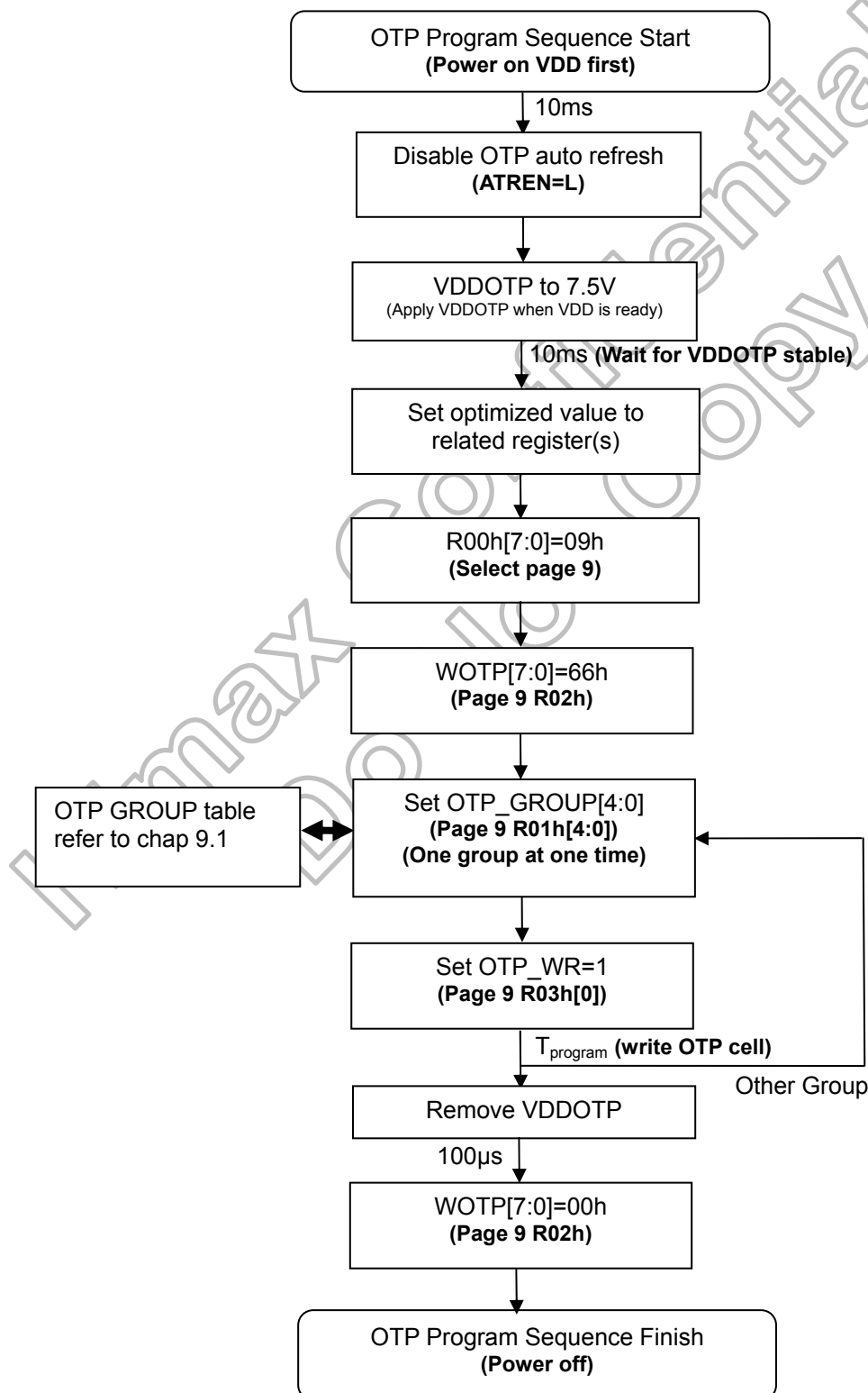
Figure 6.18: OTP 1st program sequence (OTP table1)
