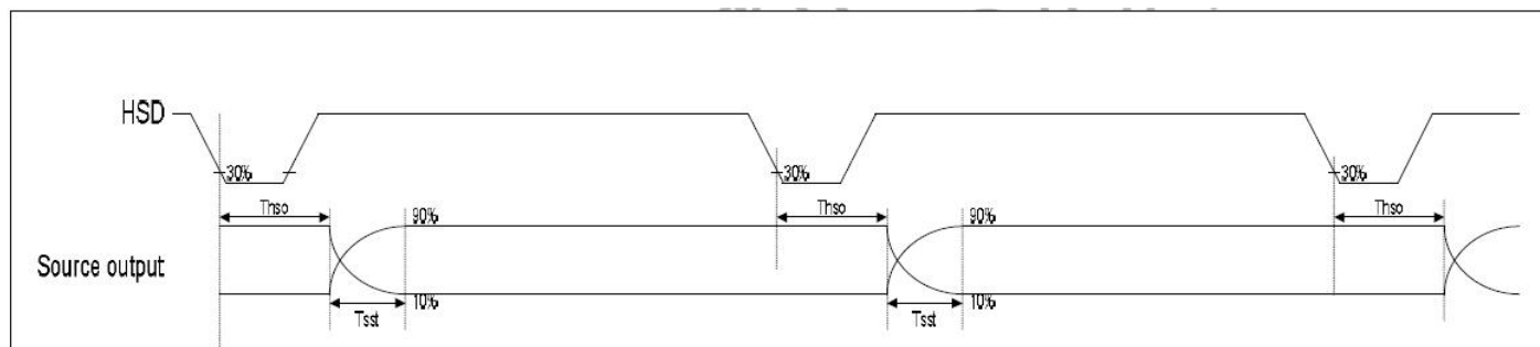
Figure 6.4.2.2.1: Source Output Timing Diagram
