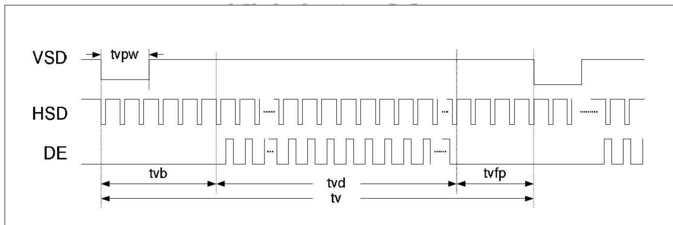
Figure 6.3.2: Vertical Input Timing Diagram
