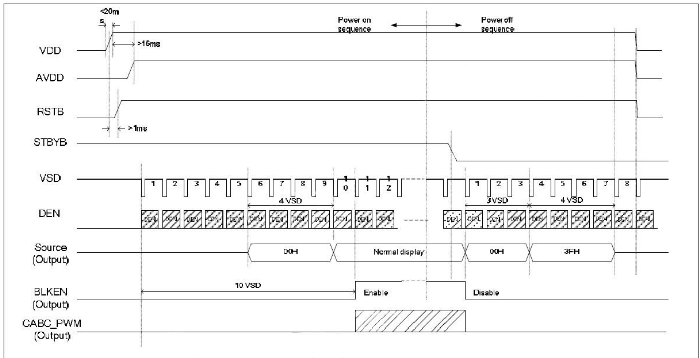
Figure 5.1.1: Power on/off Timing Sequence
