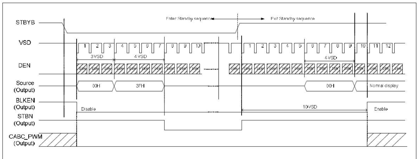
Figure 5.1.2: Enter and Exit Standby Mode Sequence
