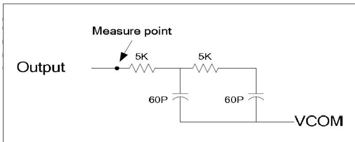
Figure 6.4.2.2.2: Output Load Condition
