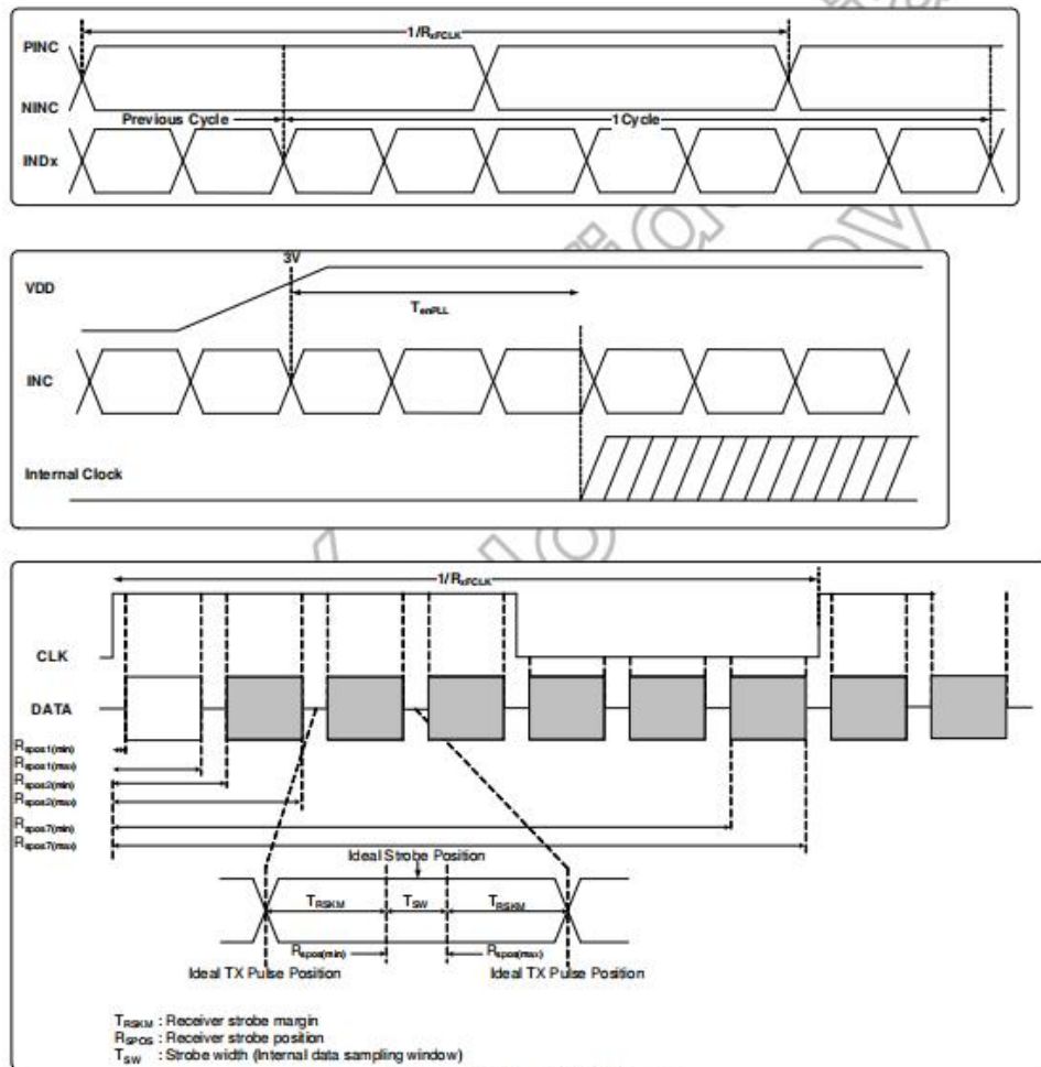
Figure 13.3: LVDS figure
