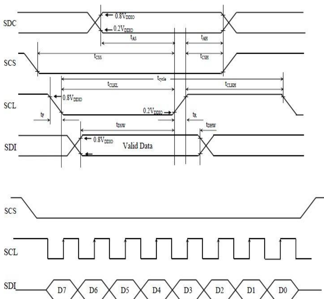
Figure 13-3: 4 wire Serial Timing Characteristics
