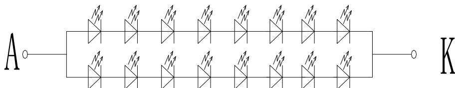
Figure: LED connection of backlight(Constant Current)
