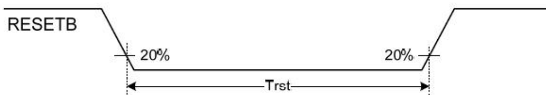
Figure 13.6: Reset timing
