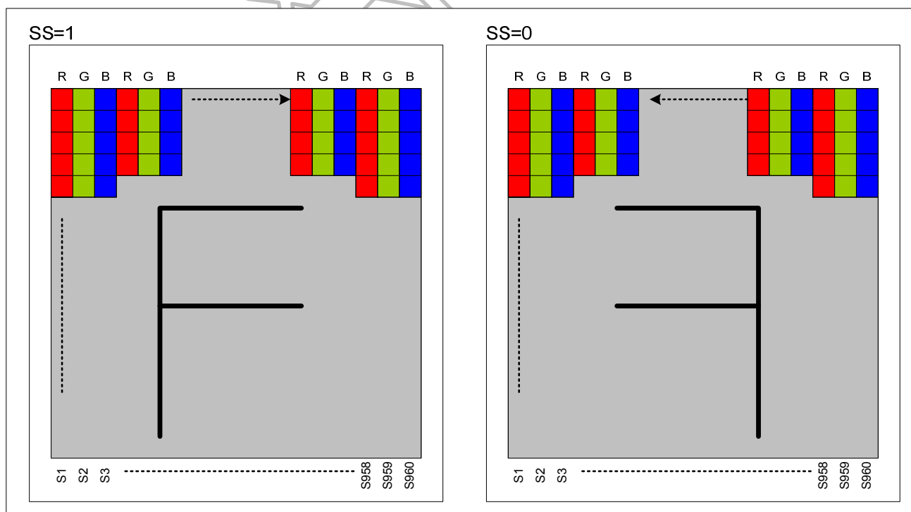
Figure 7. 26: Display direction according to SS
