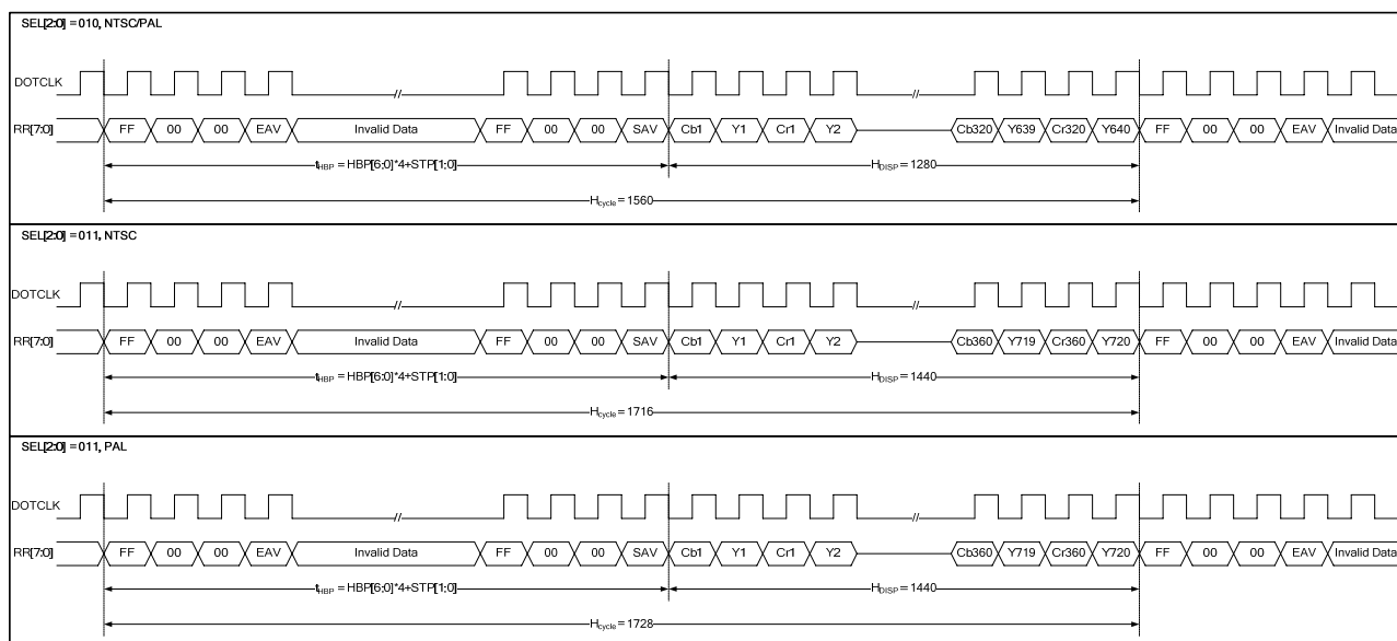
Figure 12. 8: CCIR656 horizontal timing
