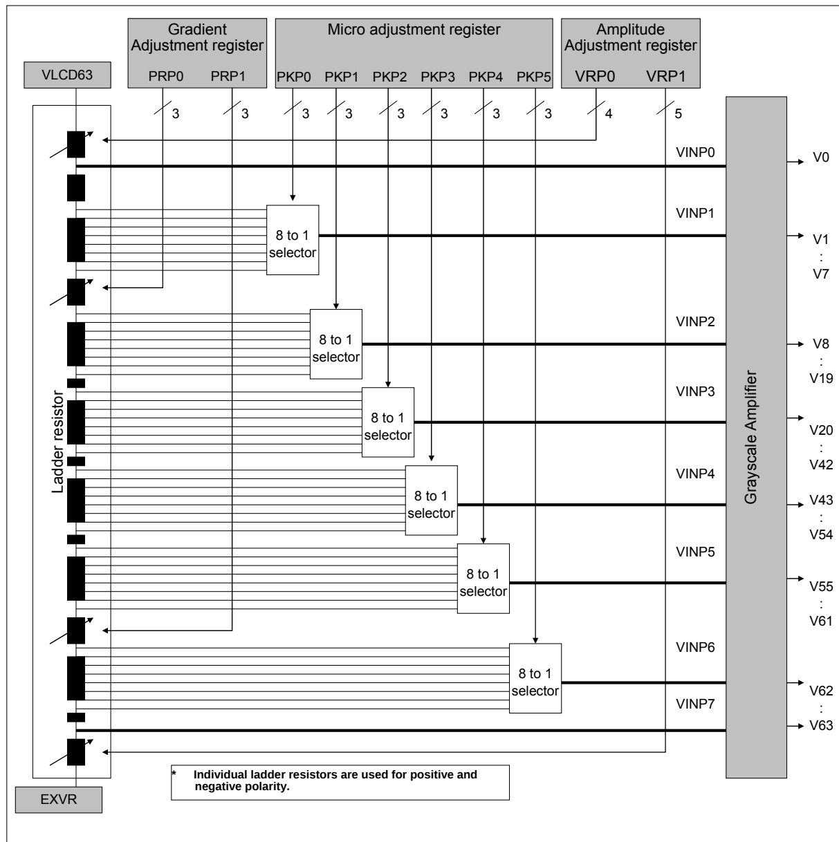
Figure 9. 2: Grayscale amplifier
