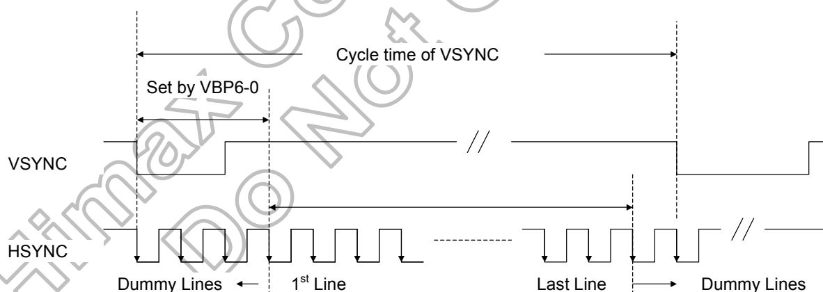
Figure 7. 20: No. of clock cycle of HSYNC
