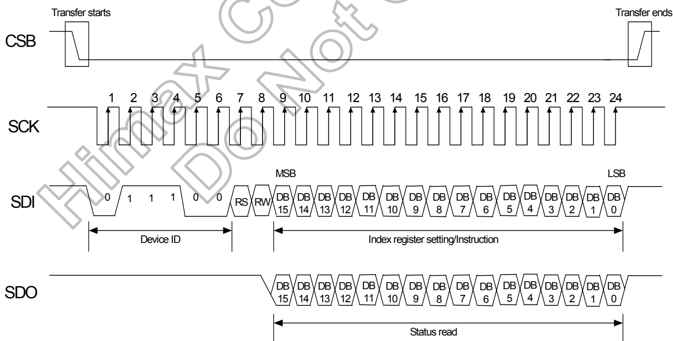
Figure 6. 1: SPI timing
