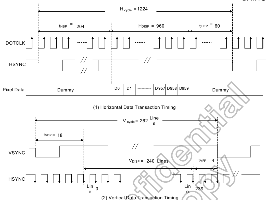
Figure 12. 3: Data transaction timing in serial RGB (8-bit) interface (SYNC mode)
