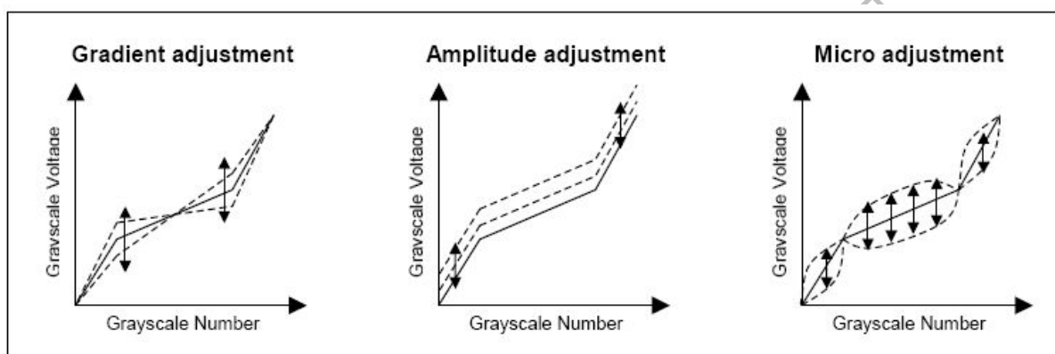
Figure 9. 4: Gamma adjustment function
