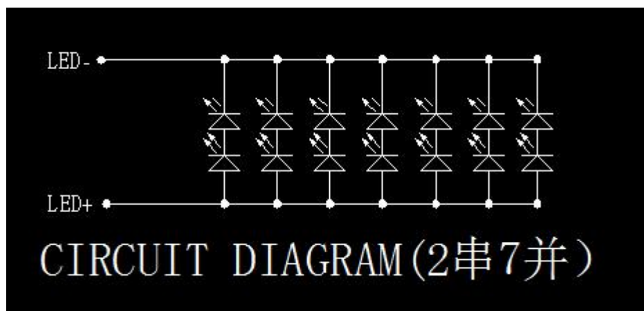
Figure: LED connection of backlight(Constant Current)
