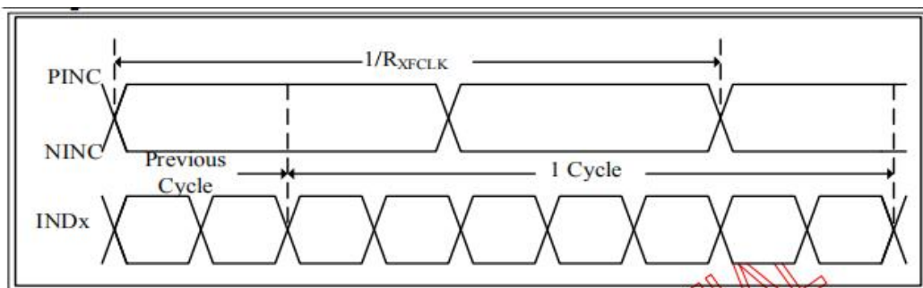
LVDS timing(1)
