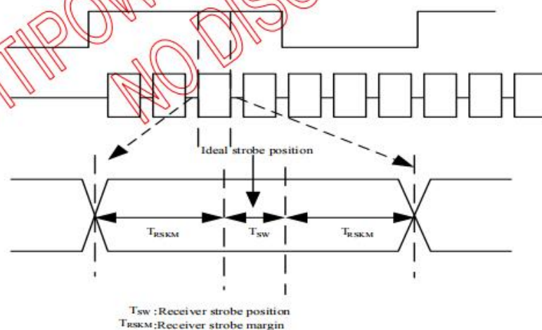
LVDS timing(2)
