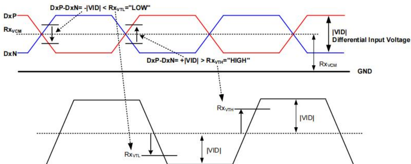
Figure 11.1: LVDS input timings
