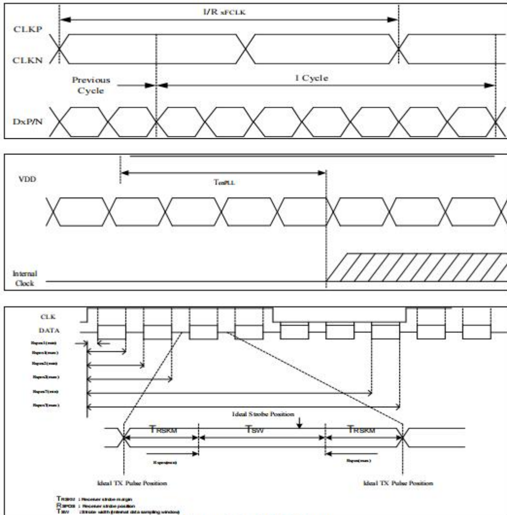
Figure 13.3: LVDS figure
