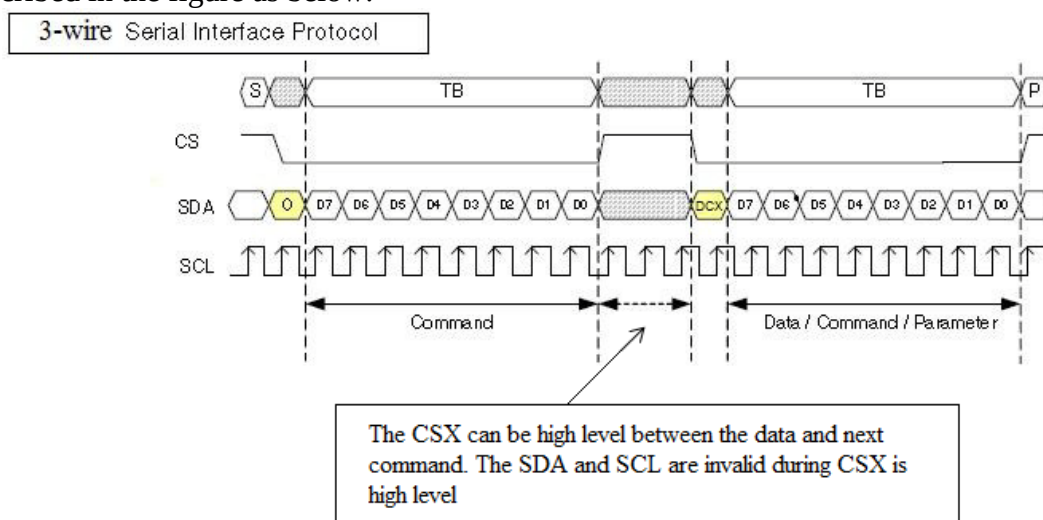
Figure 6-3-2-1-1 3-wire SPI Write Sequence
