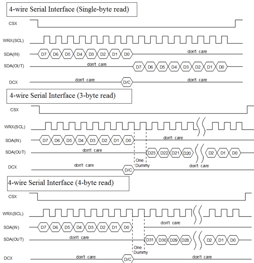
Figure 6-3-2-2-2 4-wire SPI Read Sequence
