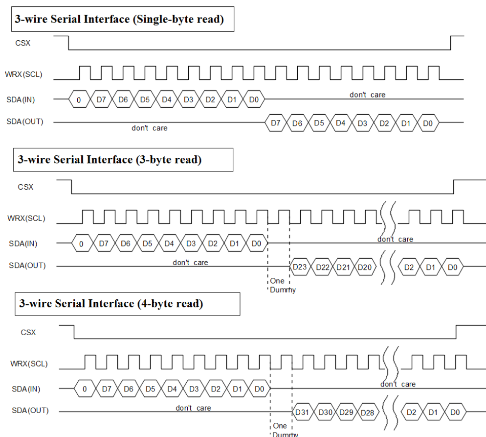
Figure 6-3-2-2-1 3-wire SPI Read Sequence
