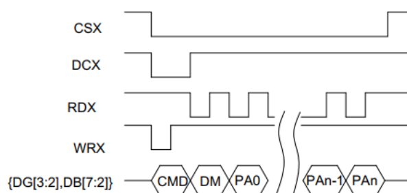
Figure 6-2-2 8080 Read sequence (8-bit parallel)
