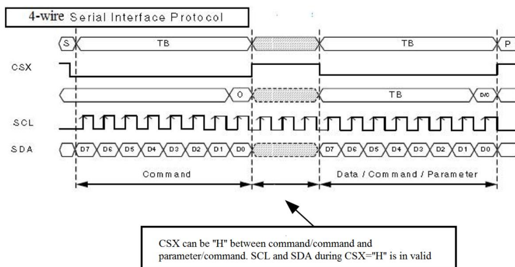
Figure 6-3-2-1-2 4-wire SPI Write Sequence
